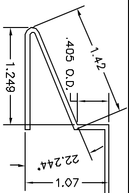
RAMP DETAIL
