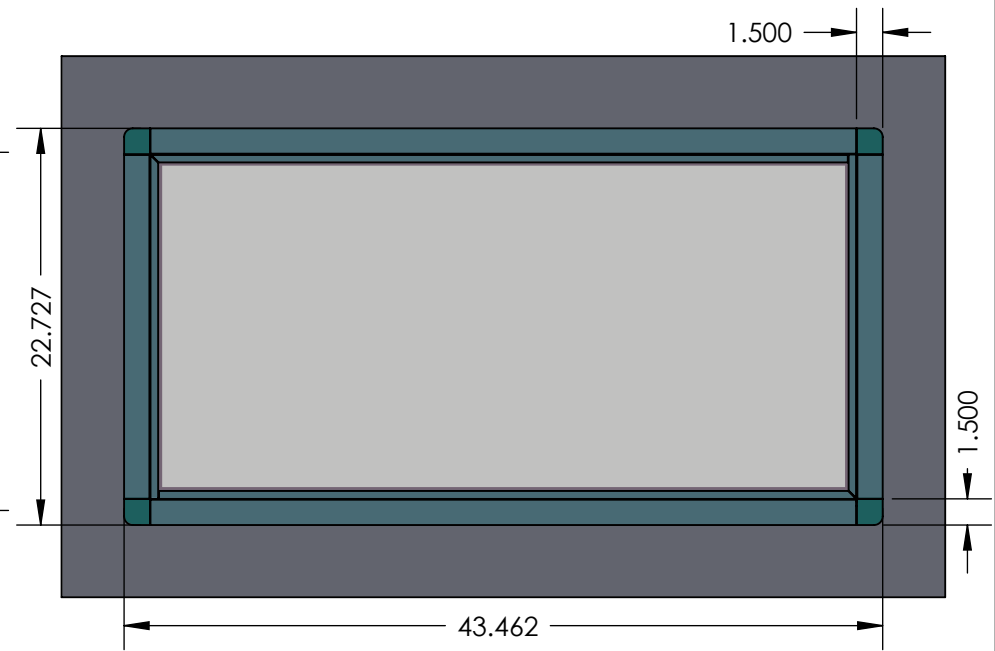
BACK VIEW
